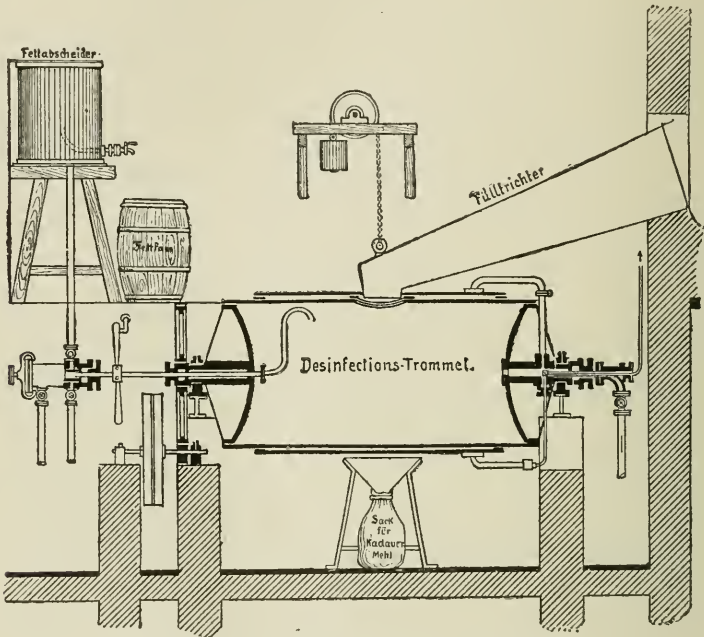
Podewils' apparatus for reducing carcasses.
